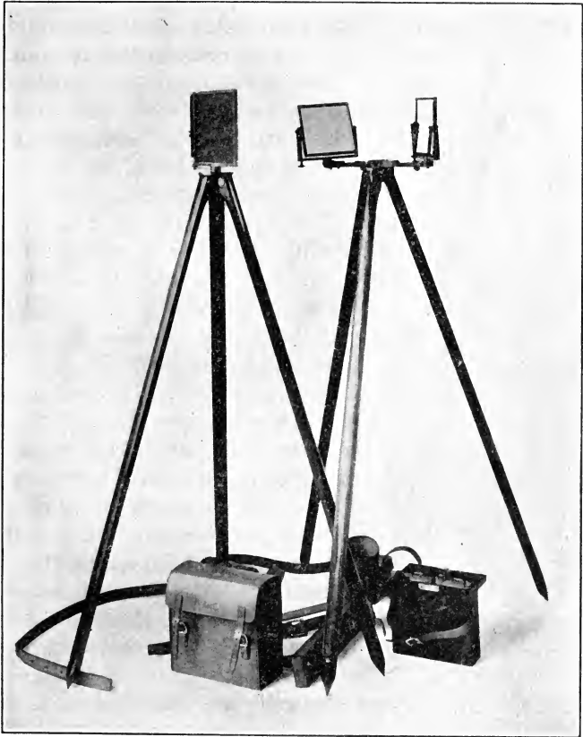
FIG. 1.—Heliograph assembled.
